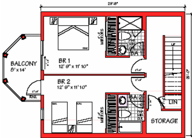
SECOND FLOOR AREA: 757 SQ FT BALCONY AREA: 94 SQ FT
